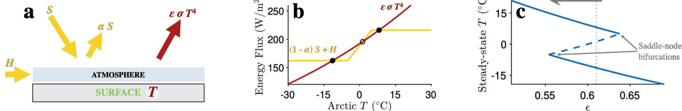
Figure 10. Simple model of how the ice-albedo feedback affects Arctic climate. (a) The main energy fluxes in the Arctic. (b) E_{in} (yellow) and E_{out} (red) in the energy balance as a function of T . Where both curves meet represent stable and unstable fixed points, which are indicated by filled and open circles, respectively. (c) Bifurcation diagram for the temperature as a function of the effective emissivity \epsilon . Increasing concentrations of atmospheric greenhouse gases cause a reduction in \epsilon .
